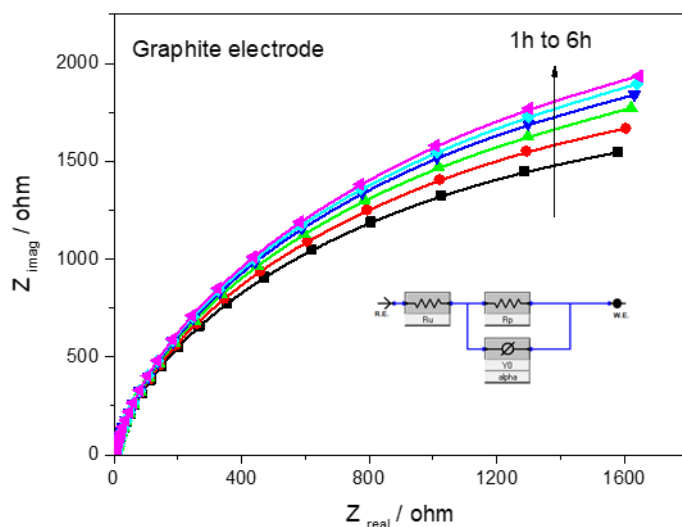
Fig. 1. Impedance measurements and equivalent scheme of the graphite support electrode at OCP in 1M H 2 SO 4 and 25°C vs. RHE
