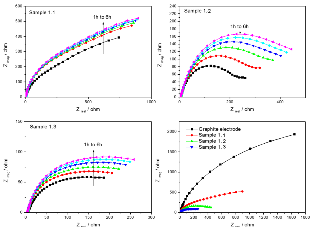
Fig. 2. Impedance measurements and equivalent scheme of the investigated samples strayed over the graphite support electrode at OCP in 1M H 2 SO 4 and 25°C vs. RHE
