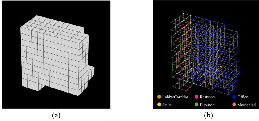
Figure 2. (a) Building Volume. (b) Voxel Graph.
