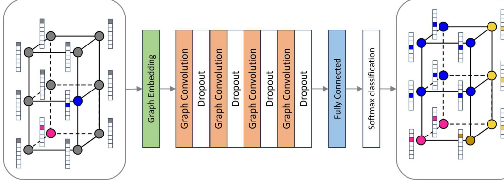
Figure 5. Structure of Graph Neural Network for Voxel Graph Dataset
