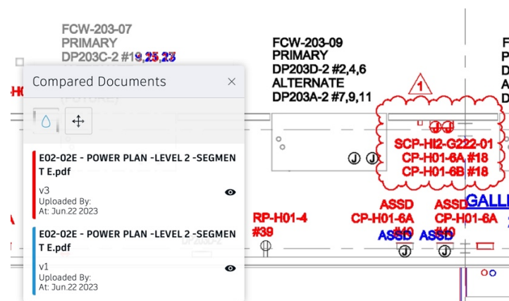
Figure 2. Overlay of Power Plan drawings comparing version 1 (issued for permit) with version 3 (issued for construction)
