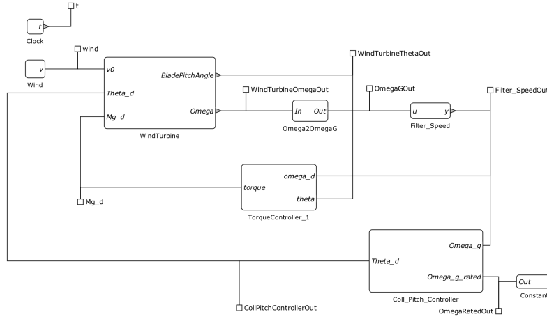
Figure 3: Wind turbine - SpaceEx model - Top Level.
