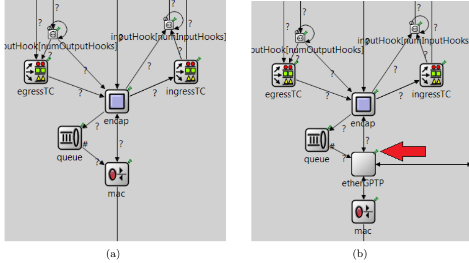
Figure 3: (a) The EthernetInterface compound module in INET, (b) the EthernetInterfaceGPTP compound module containing our etherGPTP module.
